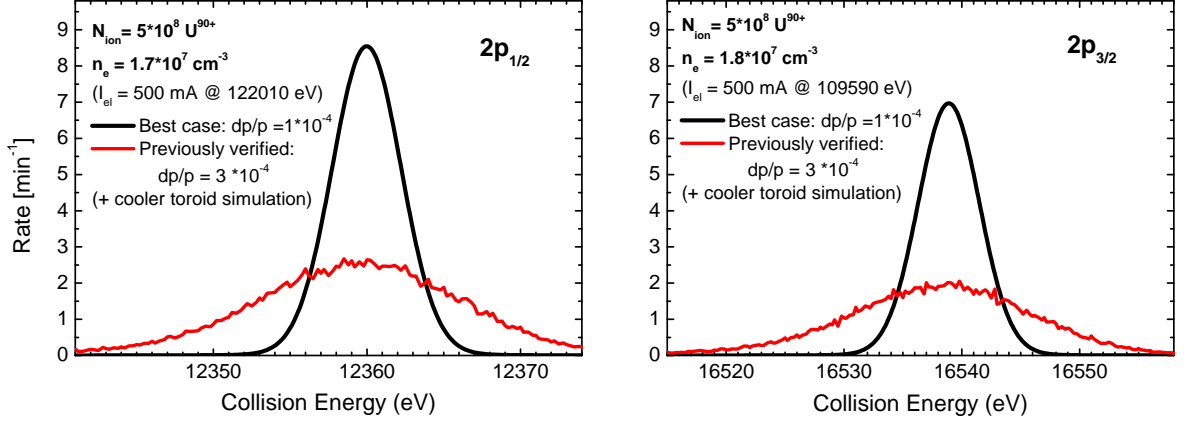
Figure 2. Total NRESX reaction rate associated with nuclear excitations 0^+ \rightarrow 2^+ and capture of the free electron into 1s^2 2p_{1/2} (left) and 1s^2 2p_{3/2} configurations (right) assuming a beam intensity of 5 \times 10^8 stored ^{238}\text{U}^{90+} ions. The black lines indicate an ion momentum spread of \delta p/p = 1 \cdot 10^{-4} which might be achieved in a best case scenario using notch-filter cooling [29]. In comparison, the red lines indicate a simulation with \delta p/p = 3 \cdot 10^{-4} which is a verified number that was achieved in previous experiments with stochastically cooled ion beams at the ESR. The latter simulation (red line) additionally takes into account the toroid sections of the electron cooler. Roughly 10 % of these products can be detected with our setup, see text. Expected beam intensities are 2 - 5 \cdot 10^8 stored ions.
