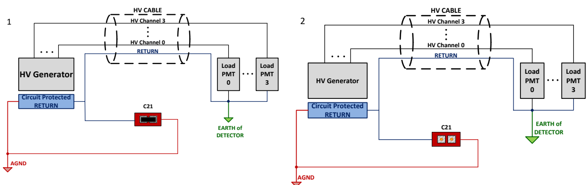
Fig. 34: Earth configuration connection examples
