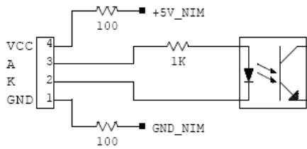
Fig. 9: KILL electrical scheme
