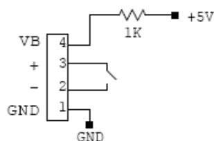
Fig. 12: ALARM electrical scheme
