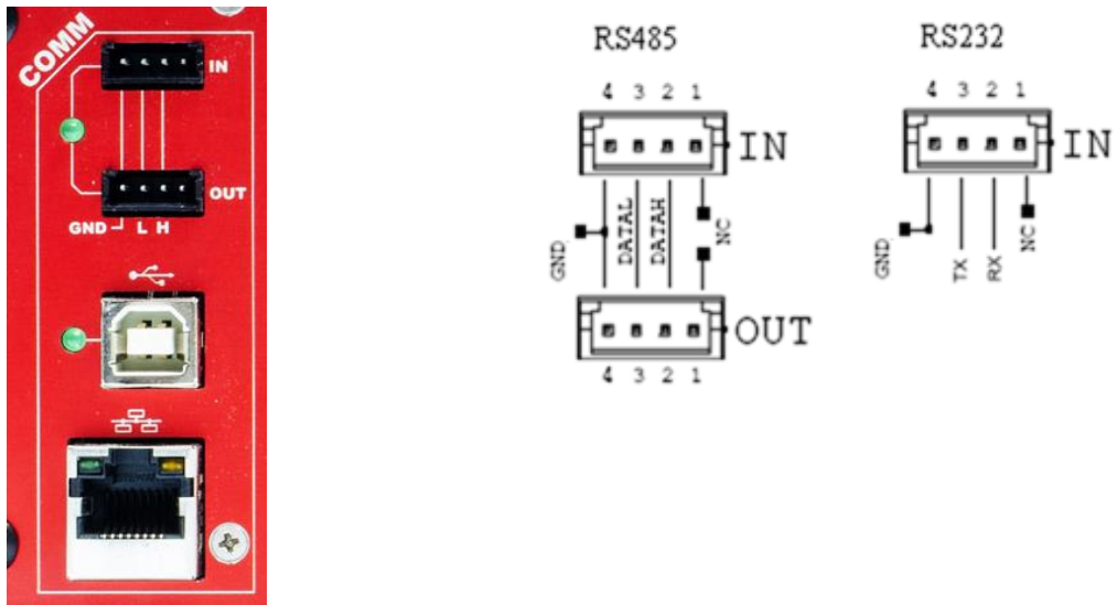
Fig. 15: Remote communication control and RS485 I/O – RS232 IN electrical scheme
