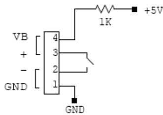
Fig. 13: ALARM TTL configured
