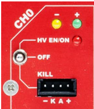
Fig. 8: Channel control panel and Kill scheme
