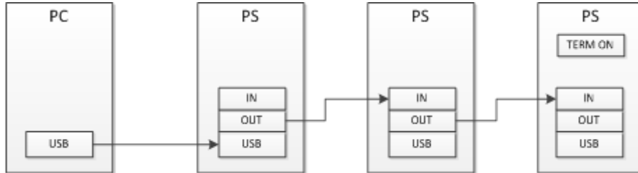
Fig. 23: USB communication diagram
