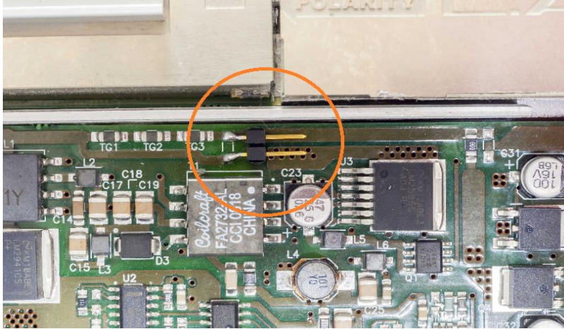
Fig. 33: C21 jumper location
