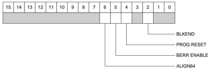
Fig. 4.16: Control Register 1
